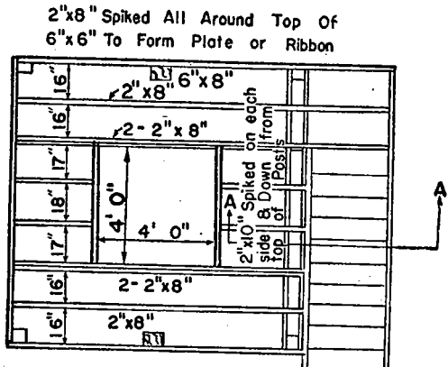
Framing For Floor \frac{1}{4}'' = 12''
