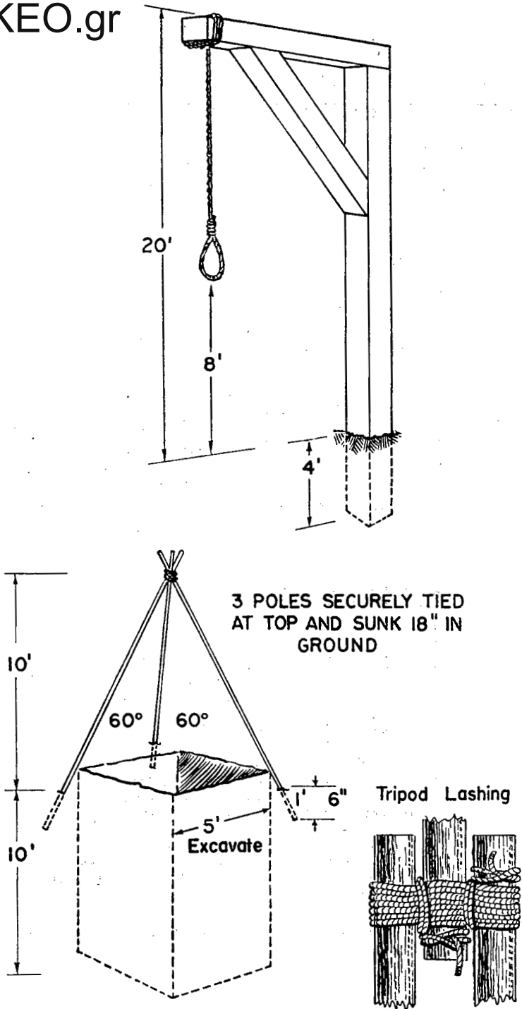
Figure 4. Emergency gallows, post type and tripod type.
